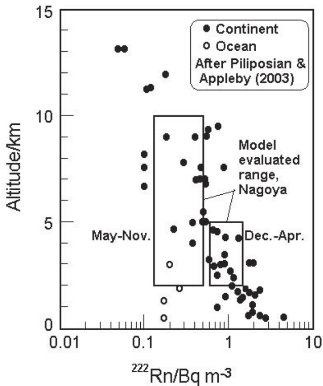
Figure 3. Comparison of observed 222 Rn concentrations over continents and a large ocean 7 with model evaluated ranges ( \pm 1\sigma ) for those in clouds, based on the data shown in Figure 2.
